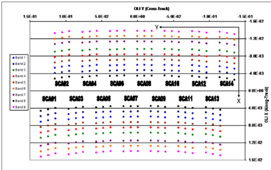
Figure A-11. OLI Line-of-Sight Coordinate System
