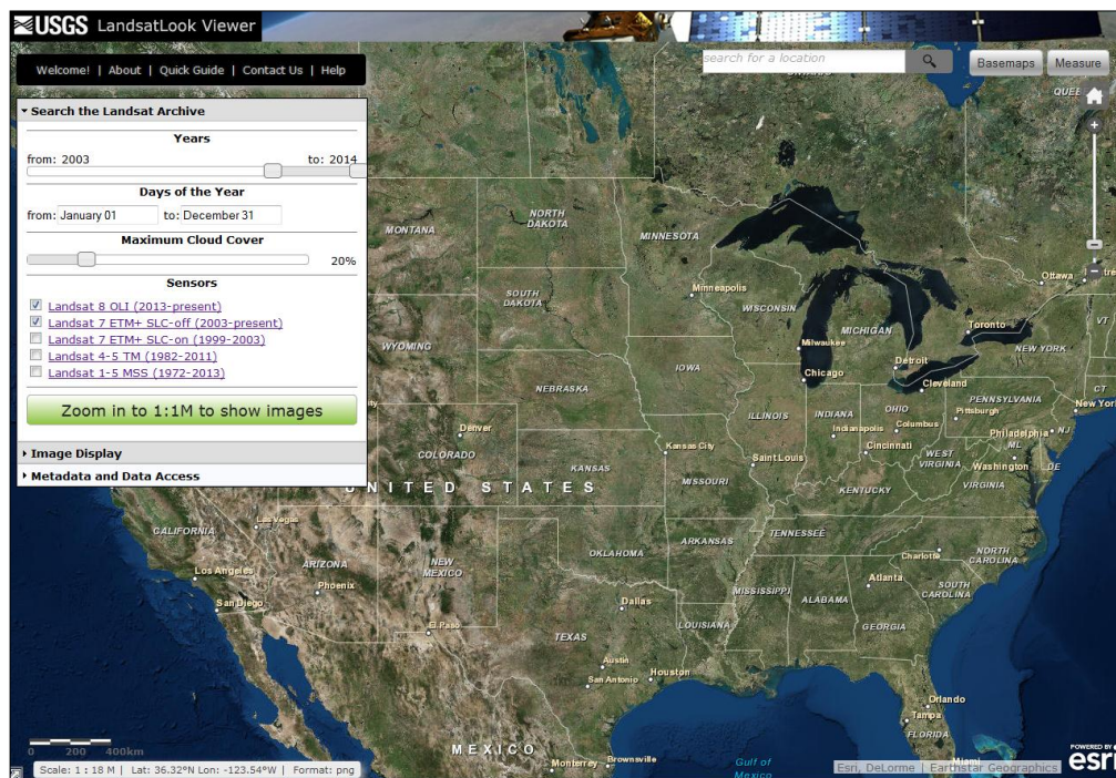
Figure 6-6. The LandsatLook Viewer
