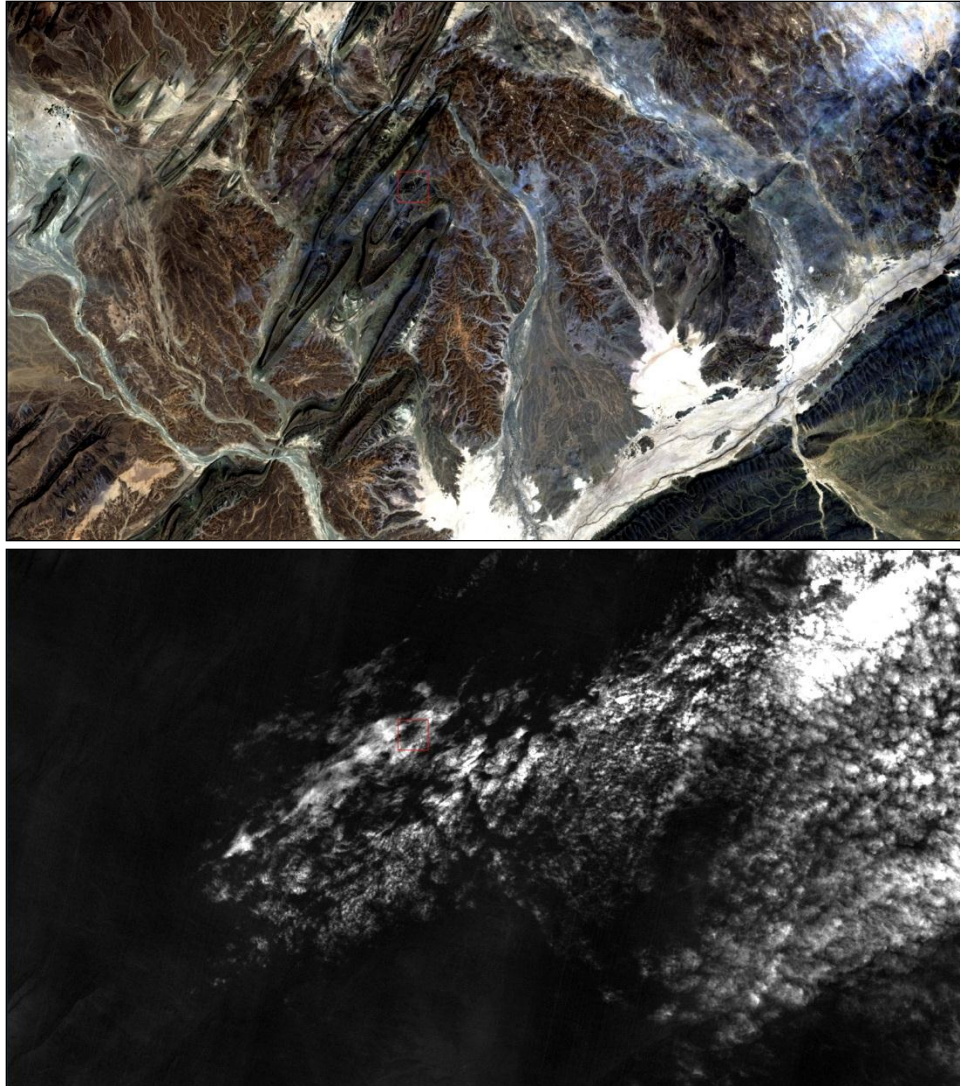
Figure 4-4. A Temperate Region Affected by Cirrus
