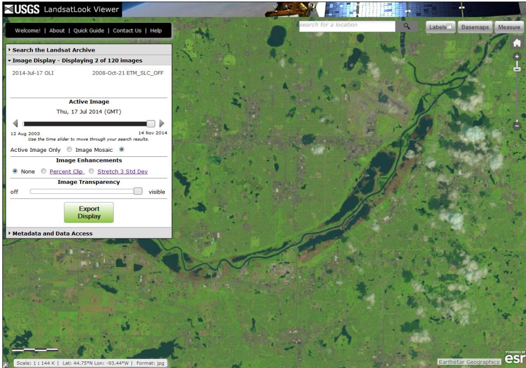
Figure 6-7. Display of Landsat Imagery
