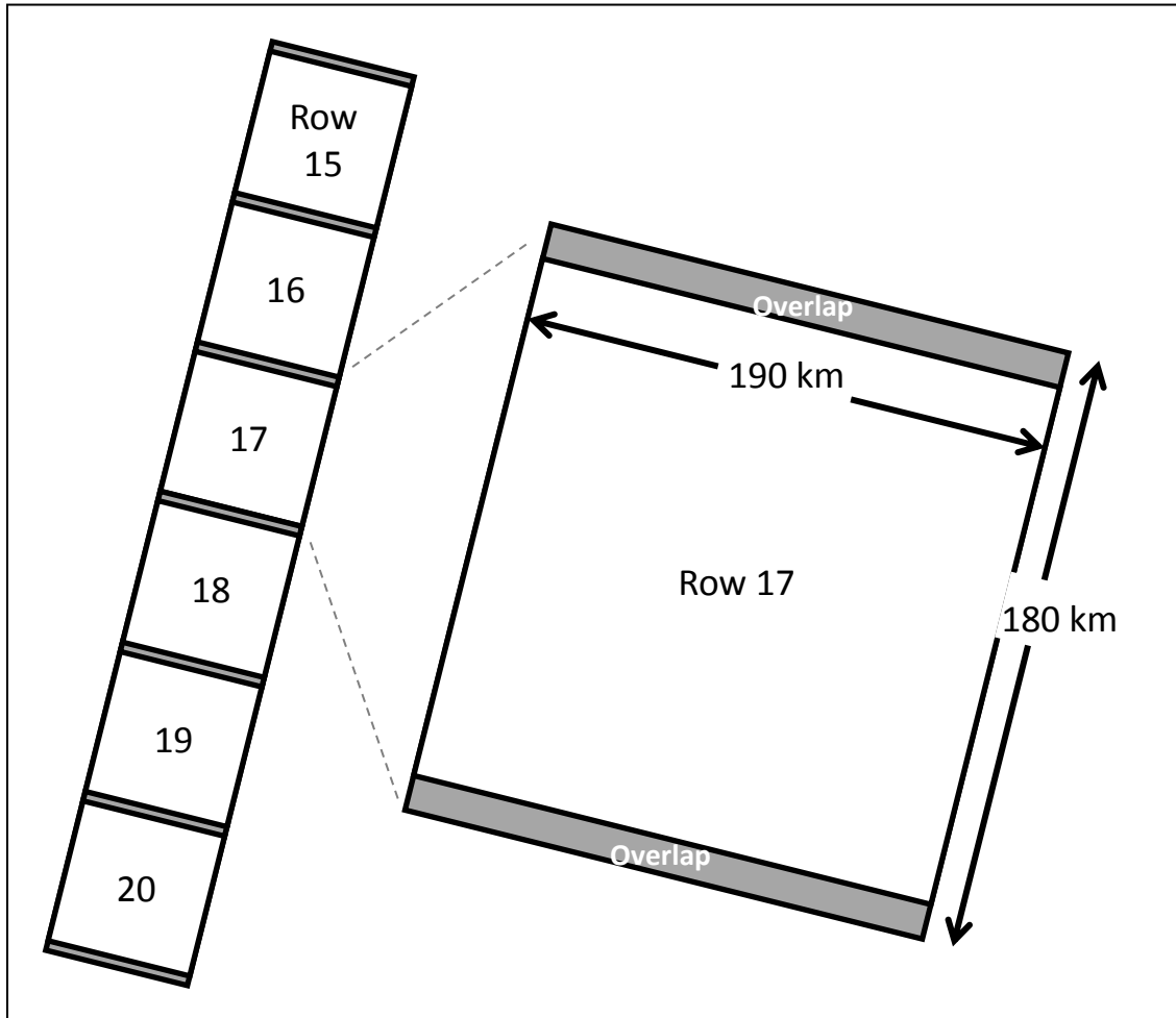
Figure 4-2. Level 1 Product Ground Swatch and Scene Size
