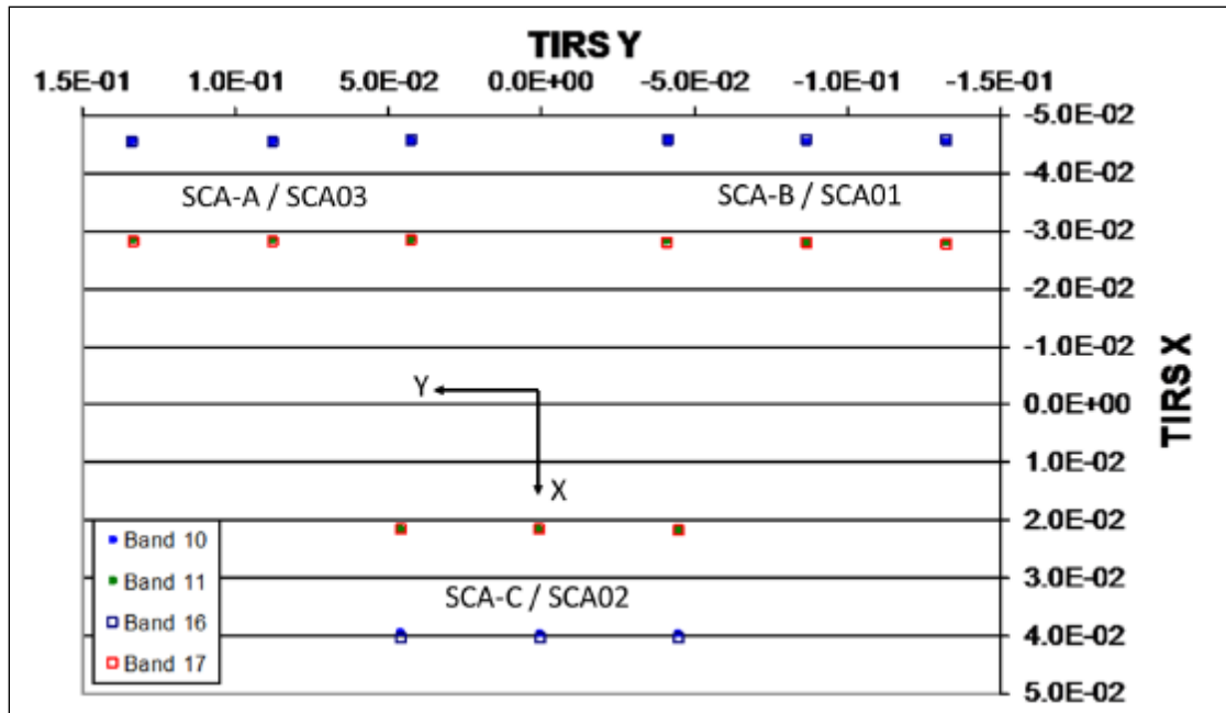
Figure A-12. TIRS Line-of-Sight Coordinates
