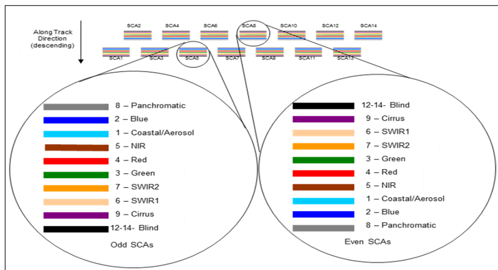
Figure 2-5. Odd/Even SCA Band Arrangement
